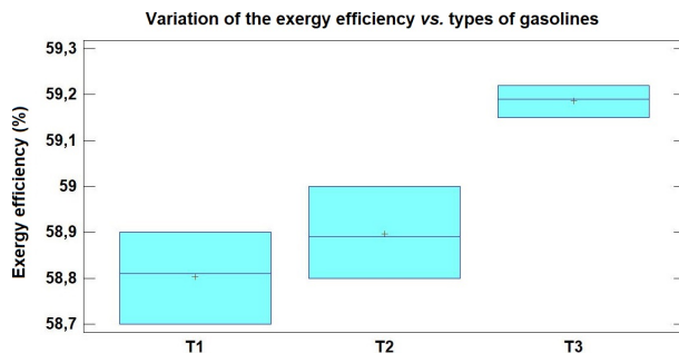
Figura 8. Comparative graph of the exergy efficiency for the different types of gasoline
