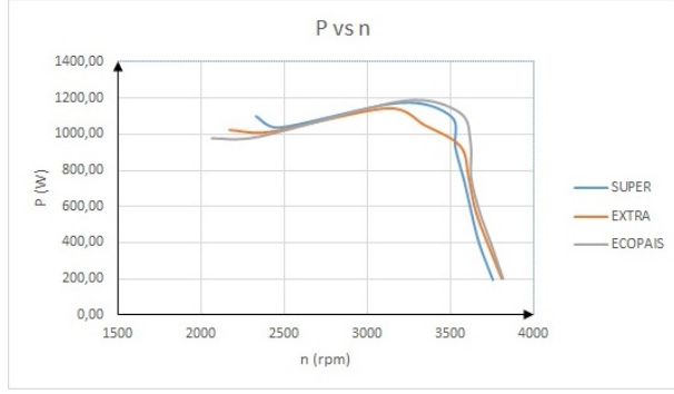
Figura 5. Curves of power vs. rpm
