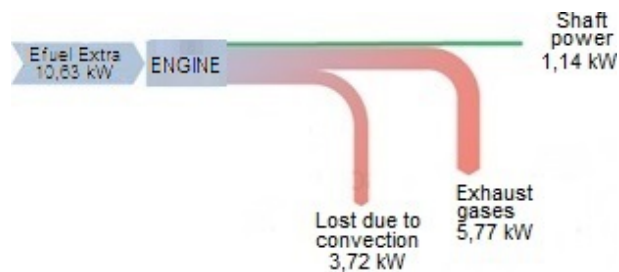
Figura 10. Sankey Diagram-Extra Gasoline
