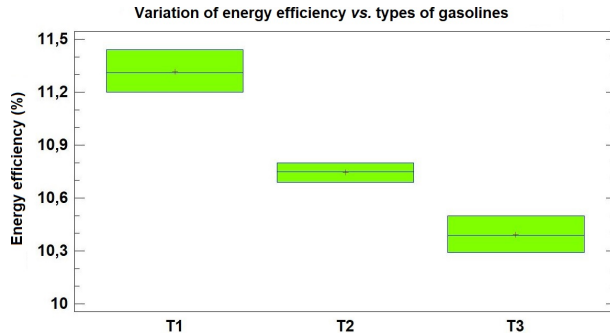
Figura 7. Comparative graph of the energy efficiency for the different types of gasoline
