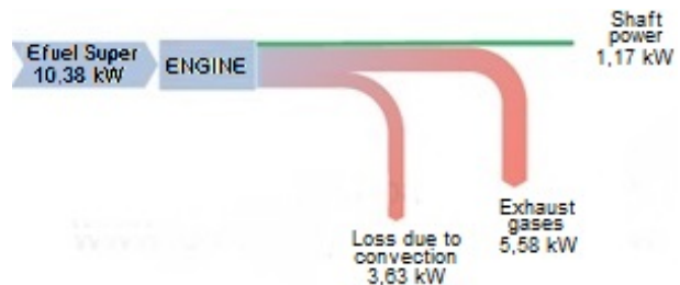
Figura 9. Sankey Diagram-Super Gasoline
