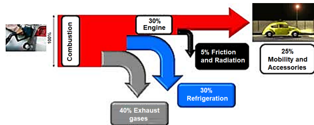
Figura 1. Sankey Diagram in ICE [17]
