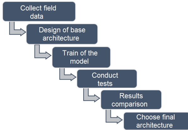
Figure 5. Methodology
