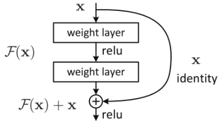
Figure 12. Block of the ResNet architecture [44]
